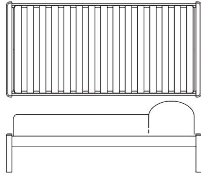
917-923R 3/3 PLATFORM BED W/SLAT PACK W41 D81 H17 (104 x 206 x 43cm)
